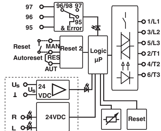
Figure 4 Block diagram
